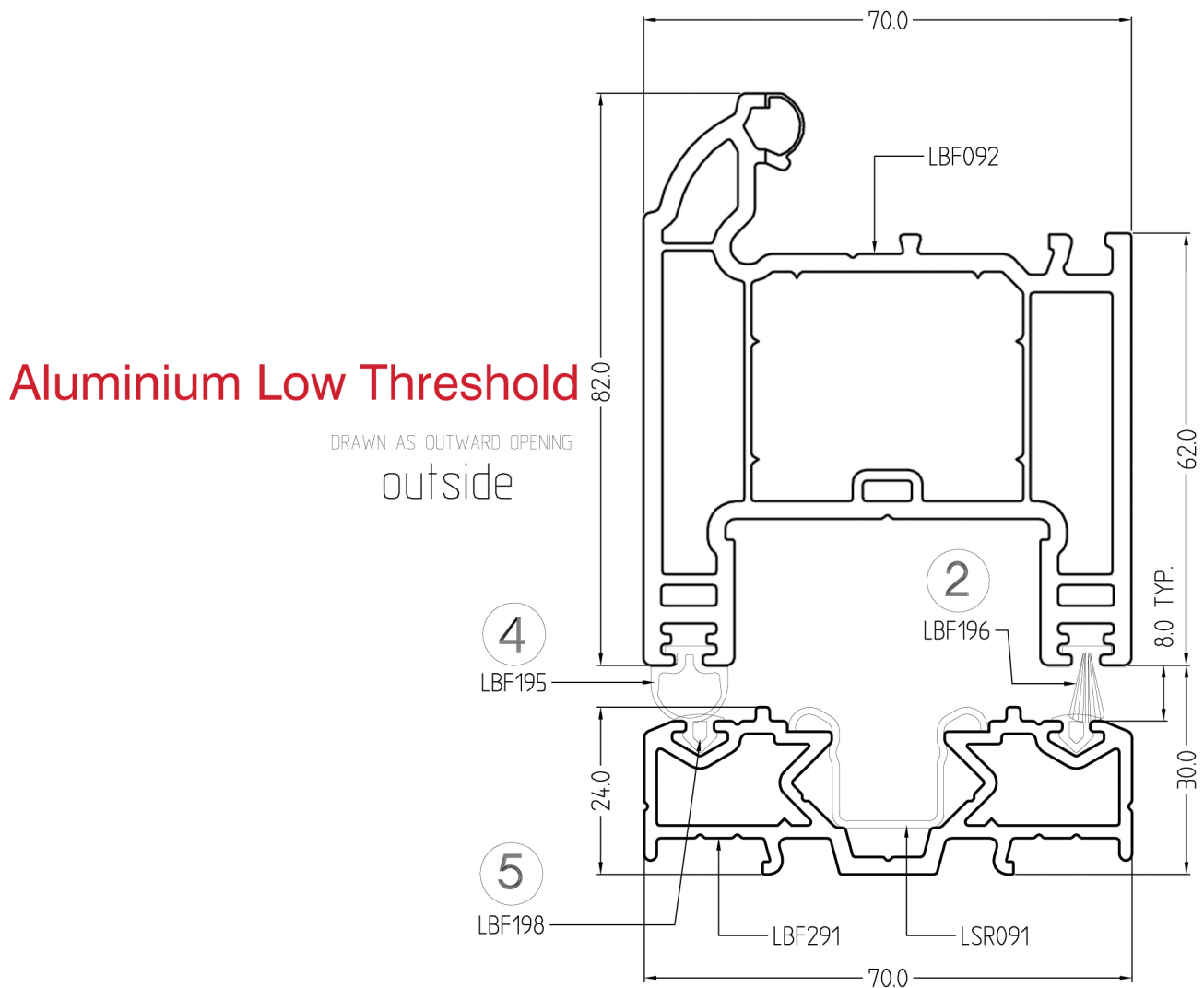
Aluminium Low Threshold Tray (Ramp)
