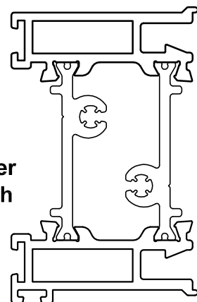
VS123 Flush Vertical Member of Bottom Sash
