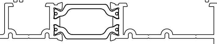
GSL1140 Head Guide Section
