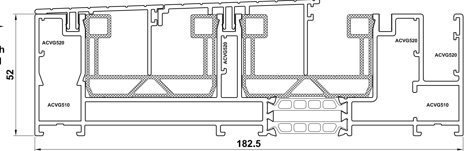
VG514 ↓ 2 Track Cover
