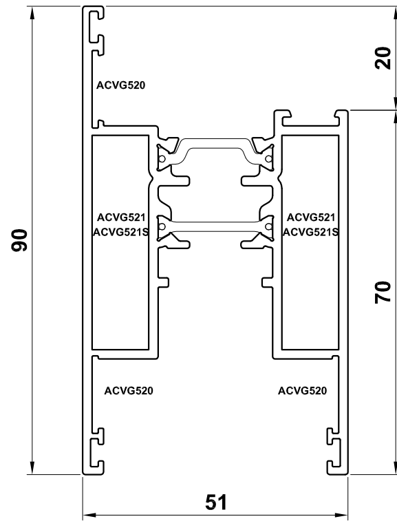
VG521 Lift & Slide Sash
