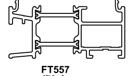
FT557 Cill Section
