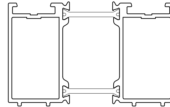
DV559 Frame Extension
