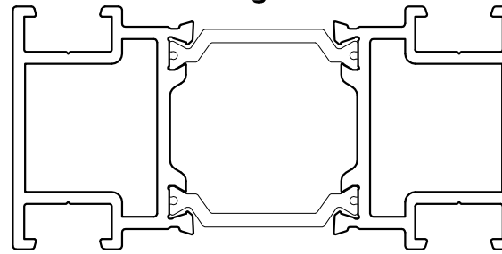
DV32 Floating Mullion
