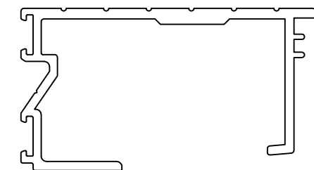
GSL1148 Internal Cill Clip Plate with Double Woolpile Carrier
