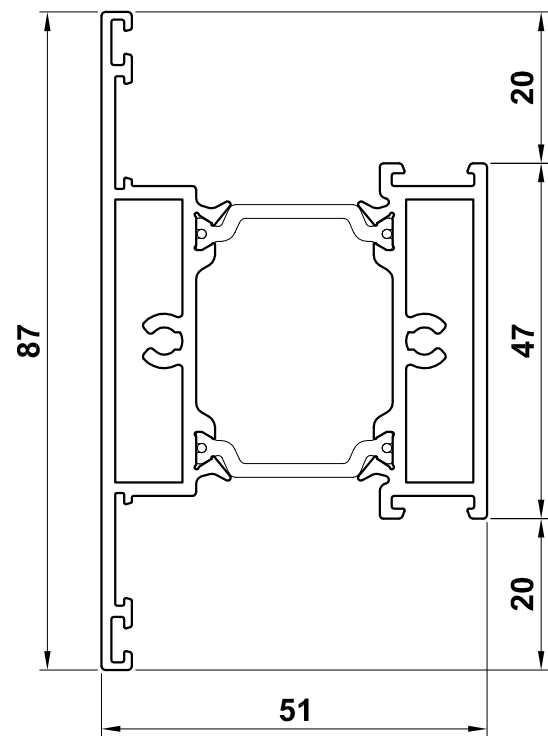
VG526 Wide Sash Transom
