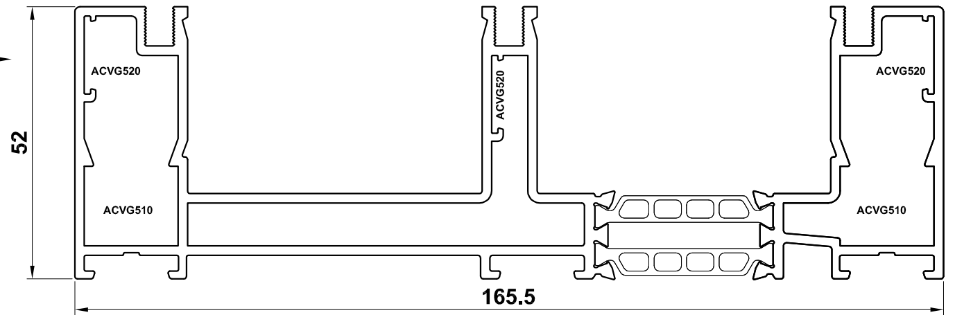
VG514 ↓ 2 Track Cover
