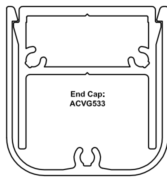
VG533 ↑ VG532 Cover Cap
