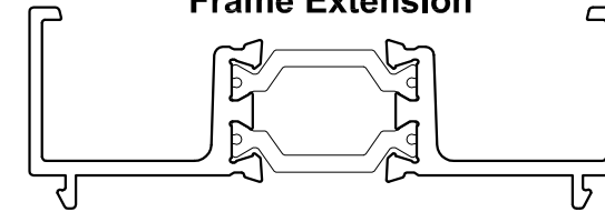
DV559 Frame Extension
