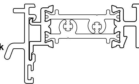
VS022 Top Rail of Bottom Sash
