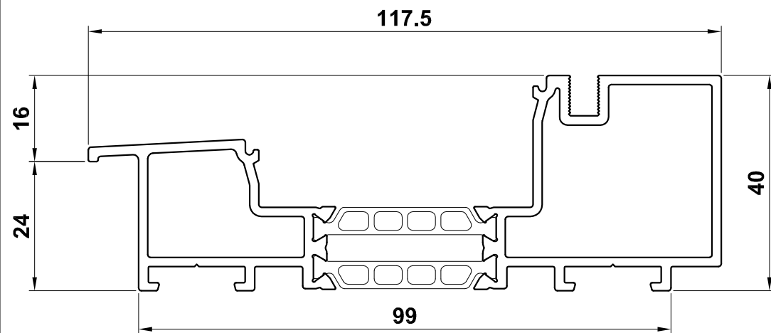
VG516 Mono Rail Threshold
