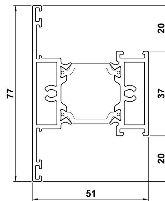
VG525 Sash Transom
