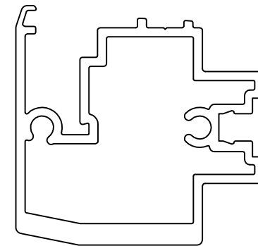
GSL1333 Three Pane Adaptor
