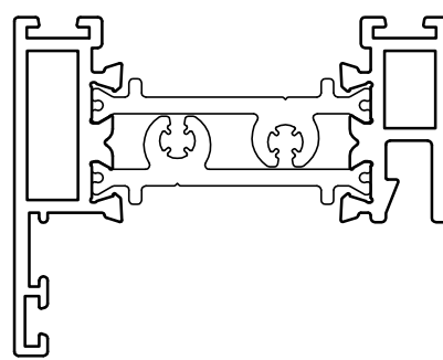
VS020 Top Rail of Top Sash & Bottom Rail of Bottom Sash
